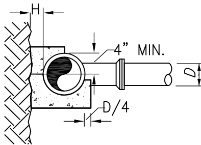
SECTION-TEE
