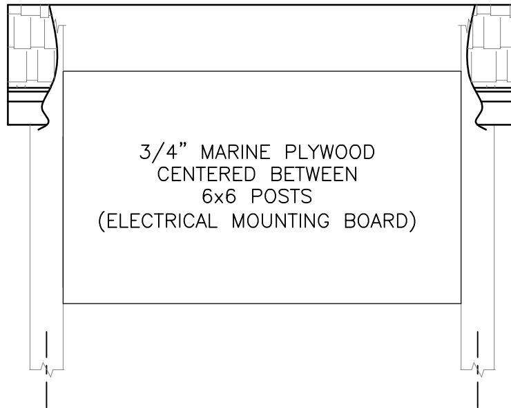
MOUNTING BOARD DETAIL
