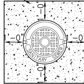
CONCRETE COLLAR PLAN
