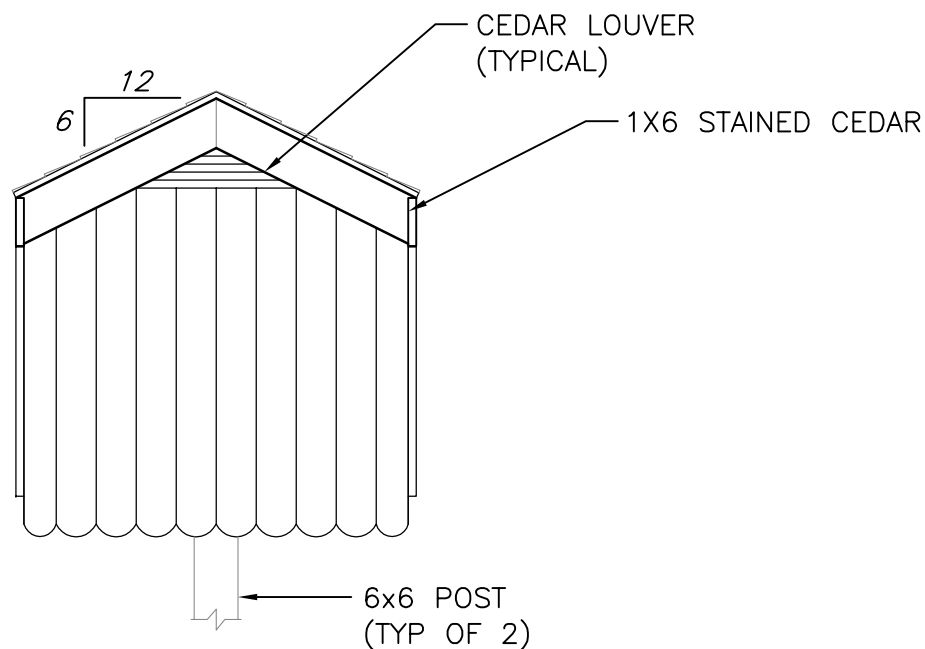
END VIEW
