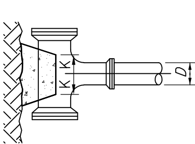
PLAN-TEE
