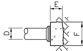
SECTION-PLUG
